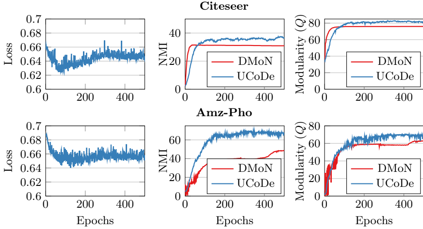
Fig. 7: Training UCoDe that quickly minimizes the loss (left); NMI increases steadily and achieves 9% (19% in Amz-Pho) higher value than DMoN (center); UCoDe gradually outperforms DMoN’s modularity (right).
