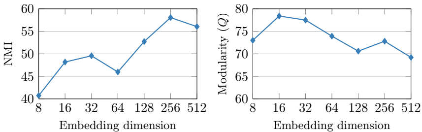
Fig. 4: Impact of the embedding dimension for non-overlapping dataset Cora (similar for other data). The maximum modularity (right) does not correspond to the best NMI (left). The optimal embedding dimension for the intermediate layer is 256.
