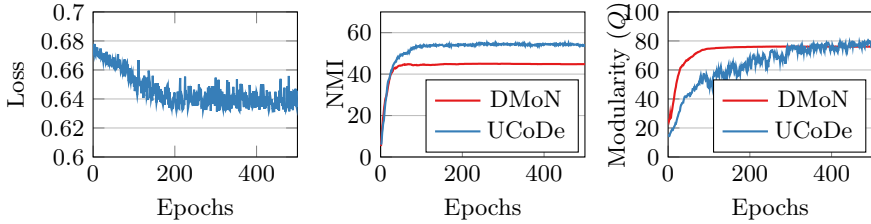
Fig. 3: Training (Cora): UCoDe quickly minimizes the loss (left); NMI increases steadily and achieves 21% higher value than DMoN (center); UCoDe gradually outperforms DMoN’s modularity (right). The alternating convergence pattern is characteristic of contrastive loss.
