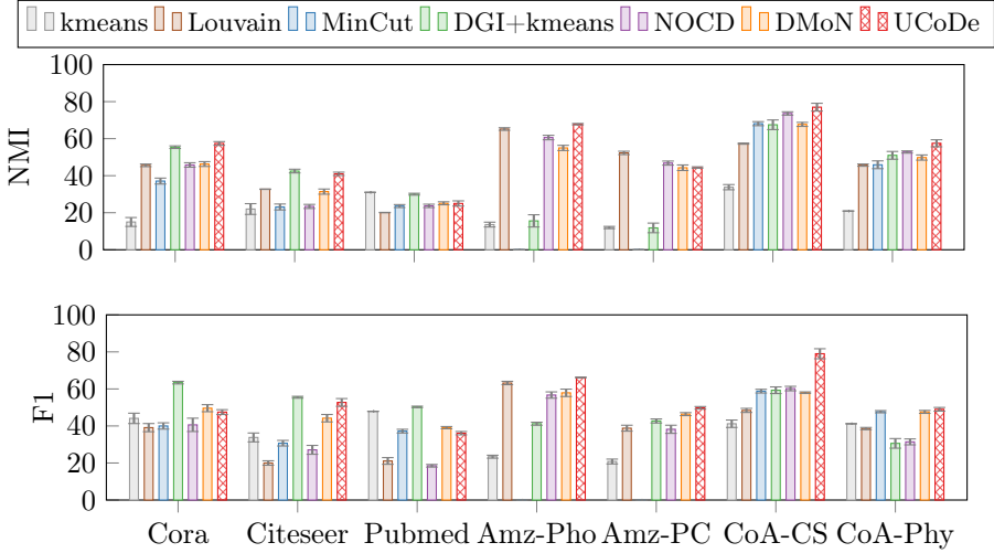
Fig. 2: NMI, F1, and confidence intervals, for non-overlapping community detection.
