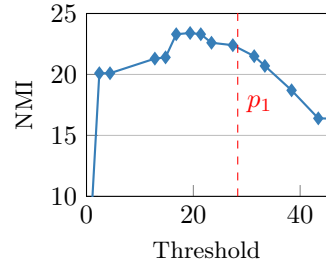
Figure 5. NMI vs. community assignment threshold; Fb-686 dataset.
